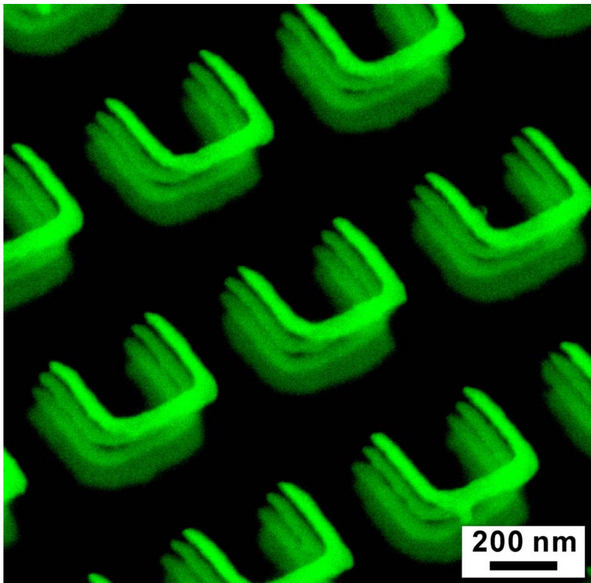
Figure 2: SEM image of the manufactured three-dimensional metamaterial, comprising 4 layers of gold split-ring resonators.
