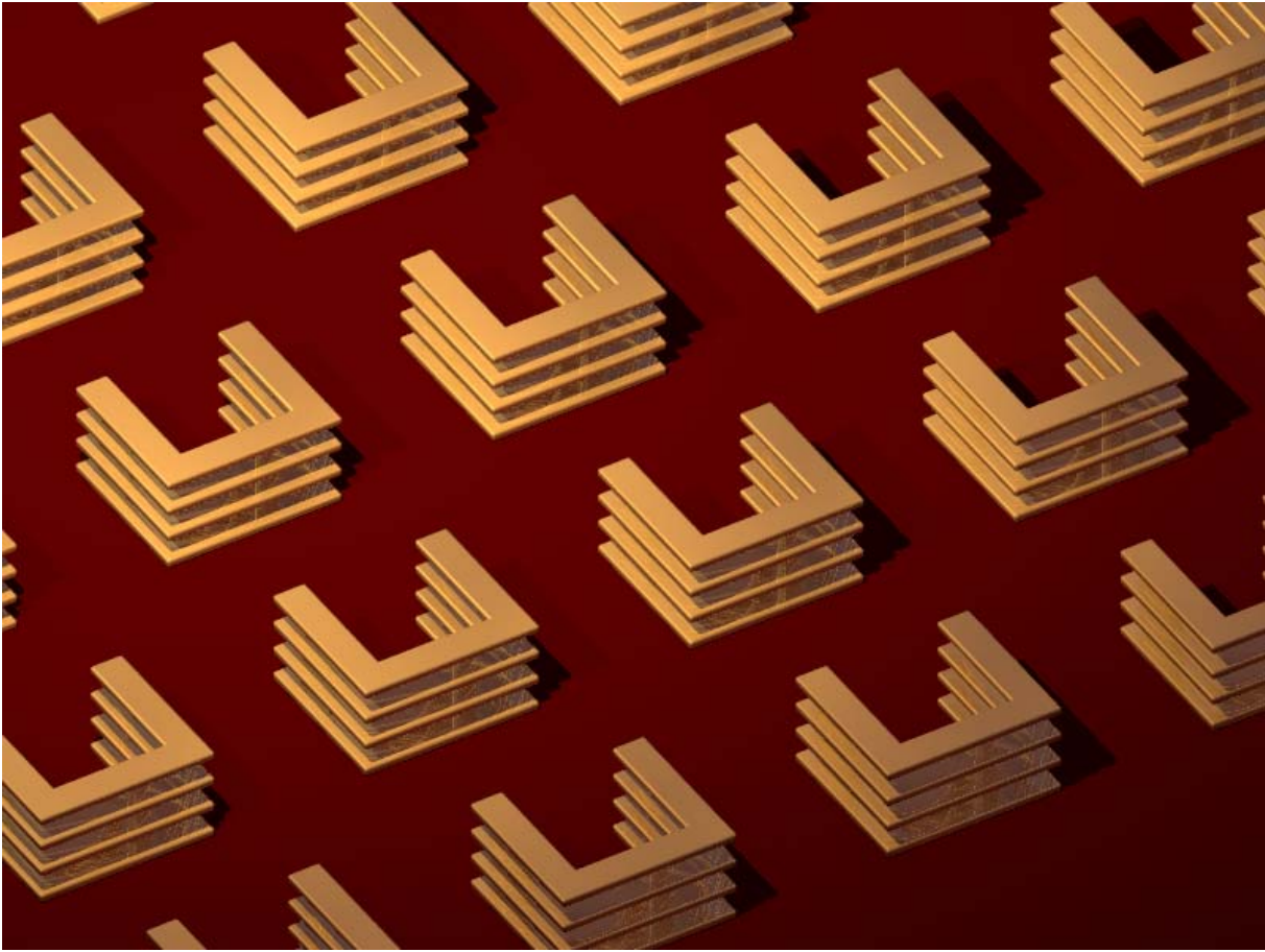
Figure 1: Concept drawing of stacked split-ring resonators made from gold and stacked on a glass substrate with polymer spacer layers.
