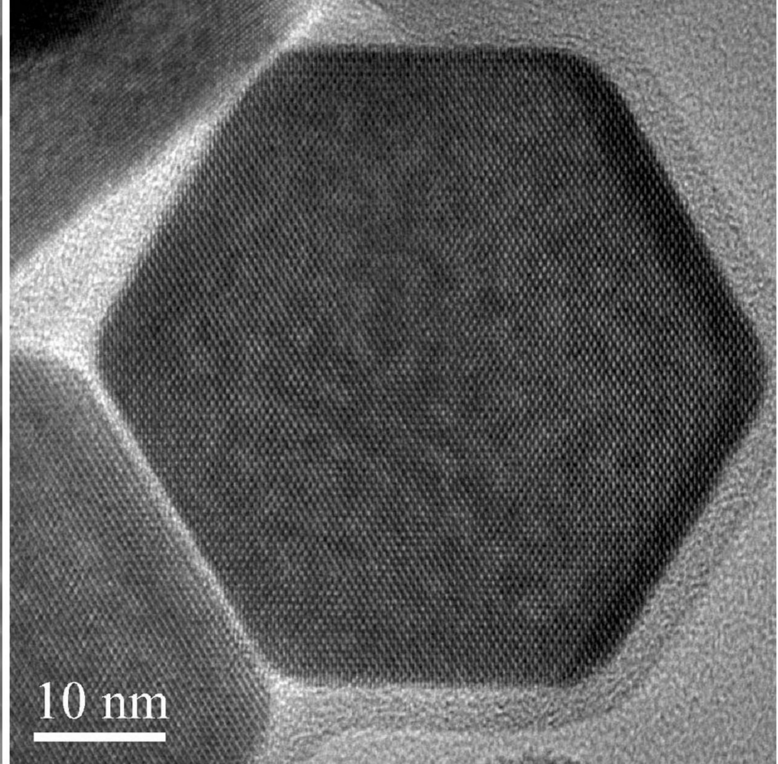
Figure 1. Transmission electron microscopy images of uniform hexagonal-phase NaYF 4 :Yb,Er upconversion fluorescent nanoplates at different magnifications. (Li ZQ, Zhang Y, Jiang S. Multicolor core/shell structured upconversion fluorescent nanoparticles. Advanced Materials 2008, 20, 4765-4769)
